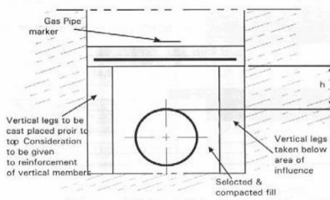
Figure 2 (b) - Concrete Slab with supports
